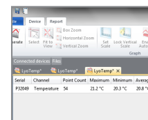
Statistics
